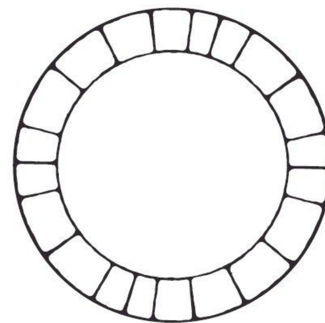
COBBLE CIRCLE RING DIAMETER: 7' 2'' JOINT WIDTH: \frac{1}{2}''
