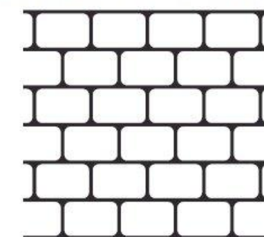
COBBLESTONE BRICK SIZE: 4 13/16" X 7 7/8" ROLL WIDTH: 33" JOINT WIDTH: 1/2"
