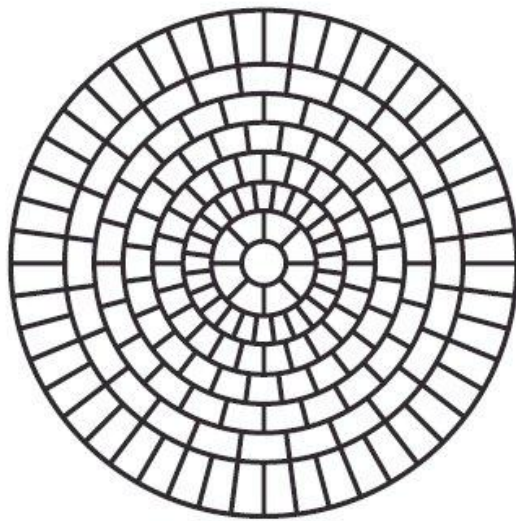
BRICK ROSETTE DIAMETER: 5' 5 \frac{1}{4}'' JOINT WIDTH: \frac{1}{2}''
