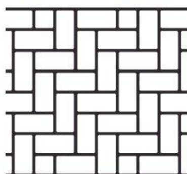
ORIGINAL HERRINGBONE BRICK SIZE: 3 3/2" X 7 3/4" ROLL WIDTH: 33 1/2" JOINT WIDTH: 1/2"
