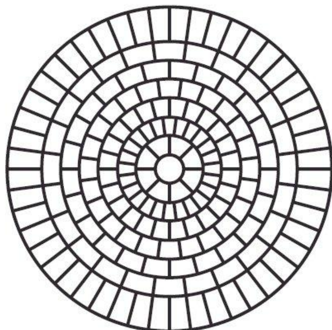
LARGE BRICK ROSETTE DIAMETER: 7' 2'' JOINT WIDTH: \frac{7}{8}''
