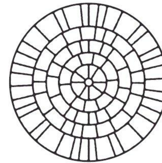
COBBLE CIRCLE DIAMETER: 5' 5'' JOINT WIDTH: \frac{1}{2}''
