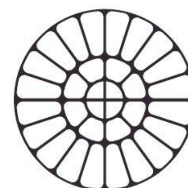
UNIVERSAL CIRCLE* DIAMETER: 2' 11 \frac{1}{2}'' JOINT WIDTH: \frac{1}{2}''
